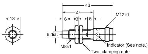
E2A-S08KN04-M1-□□
