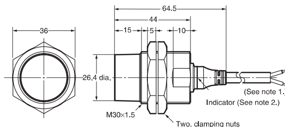
E2A-M30KN20-WP-□□/E2A-S30KN20-WP-□
