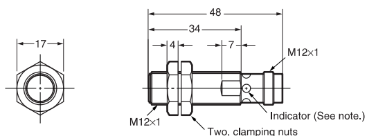
E2A-M12KS04-M1-□□/E2A-S12KS04-M1-□
