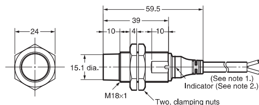
E2A-M18KN16-WP-□□/E2A-S18KN16-WP-□
