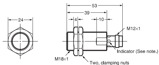
E2A-M18KS08-M1-□□/E2A-S18KS08-M1-□
