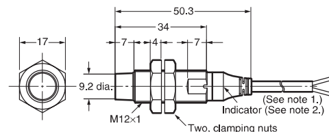
E2A-M12KN08-WP-□□/E2A-S12KN08-WP-□
