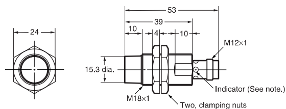
E2A-M18KN16-M1-□□/E2A-S18KN16-M1-□
